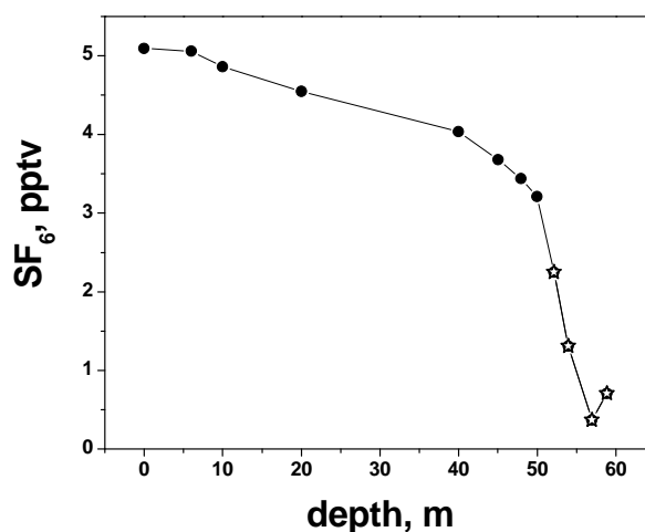
Fig. 4. Profile of SF 6 at Berkner measured by MPI-Chemistry, Mainz (circles) and by University of Heidelberg (stars). The increase near COD indicates contamination by ambient air, most likely due to compressor leakage. Error bars are smaller than the symbol size.
