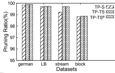
Fig. 15. Pruning Ratio vs. Datasets
