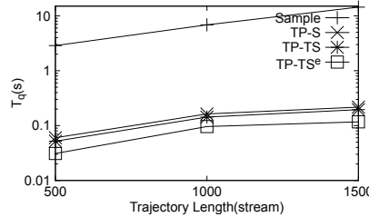
Fig. 18. T_q vs. Query Length
