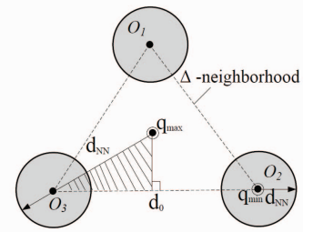
Fig. 11. \Delta -neighborhood
