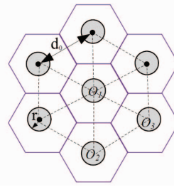
Fig. 10. Hexagonal Model
