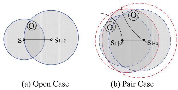
Fig. 8. Open Case and Pair Case
