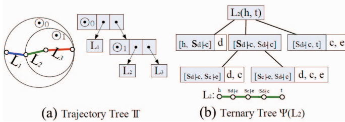
Fig. 6. Trajectory Tree \mathbb{T}(\mathcal{T}) and Ternary Tree \Psi(L_2)
