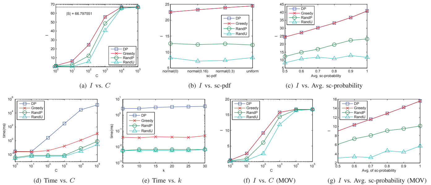
Fig. 6. Effectiveness and Efficiency of Cleaning Algorithms.
