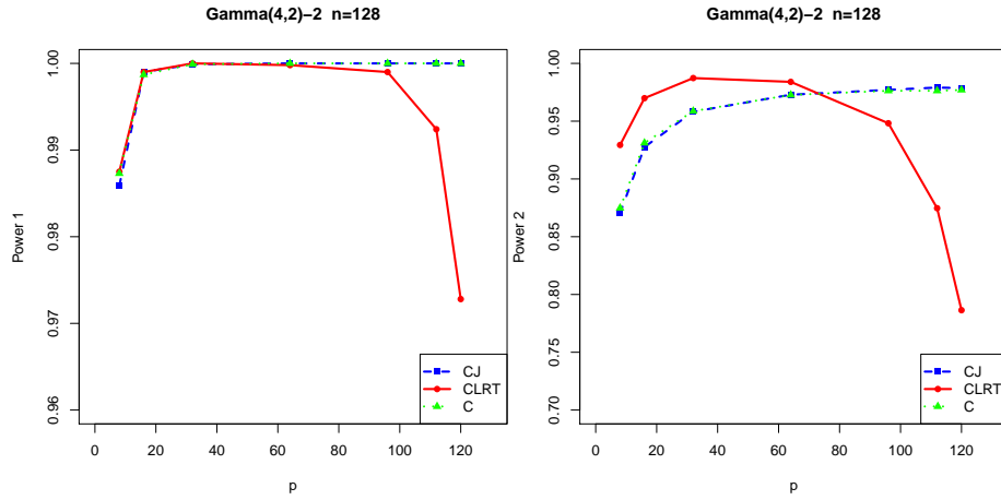
FIG 2. Empirical powers of CJ, CLRT and C test at 5% significance level based on 10000 independent applications with real \text{Gamma}(4,2)-2 random variables for fixed n = 128 under two alternatives Power 1 and 2 (see the text for details).
