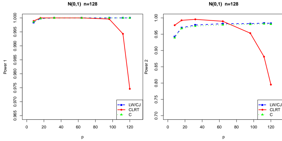
FIG 1. Empirical powers of LW/CJ, CLRT and C test at 5% significance level based on 10000 independent applications with real N(0,1) random variables for fixed n = 128 under two alternatives Power 1 and 2 (see the text for details).
