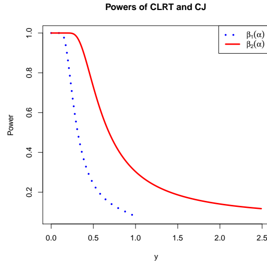
FIG 3. Theoretical powers of CLRT ( \beta_1(\alpha) ) and CJ ( \beta_2(\alpha) ) under the spiked population alternative.
