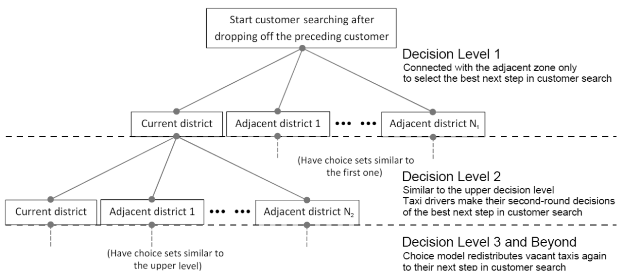
Figure 2. Decision tree of our proposed sequential logit model
