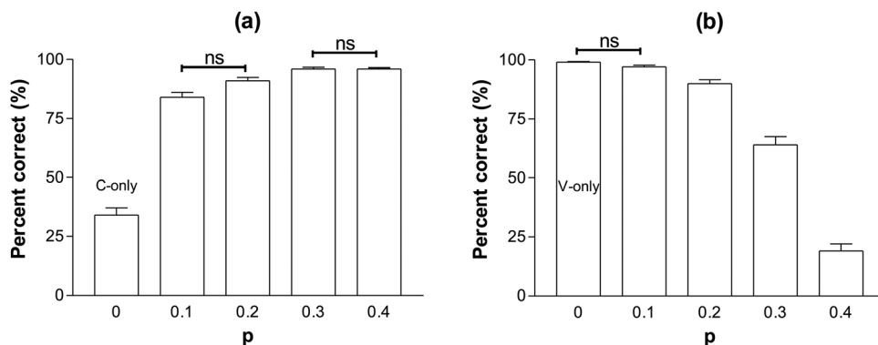
Fig. 2. Mean Mandarin sentence recognition scores as a function of proportion factor p in (a) the C + VP condition and (b) the V-VP condition. The error bars denote 1 standard error of the mean. ns, the difference of paired intelligibility scores is not significant ( p > 0.005 ).
