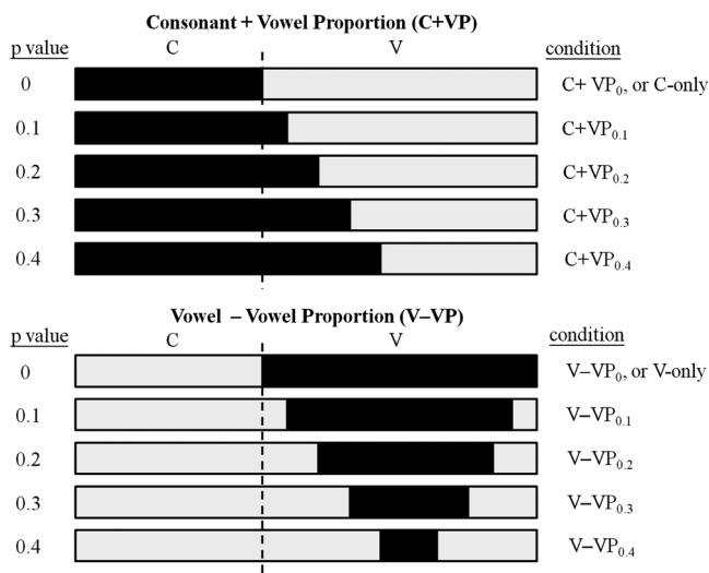
Fig. 1. Schematic of the C + VP and V-VP noise-replacement conditions for a Mandarin word. Dashed line displays the boundary between consonant and vowel. Black bars indicate the speech portions presented, and white bars indicate noise-replaced portions.
