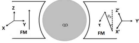
Figure 1. The schematic plot of the spin-degenerated quantum dot connected by two ferromagnetic leads. The magnetic moment of the left lead is always at z direction and the magnetic moment of the right lead is at an angle \theta_R with respect to the z -axis in the x - z plane.
