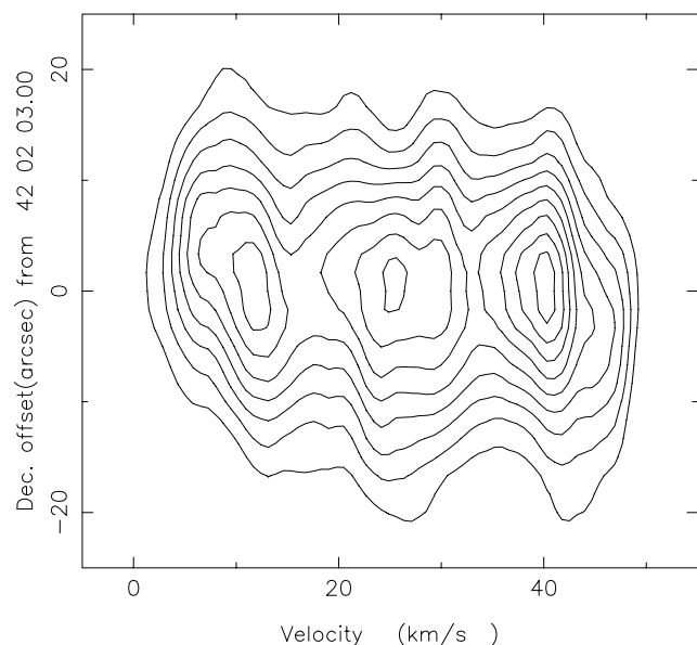
FIG. 8.—Declination-velocity map in CN ( N = 3-2 , J = 7/2-5/2 ). This is an average over -10'' \leq \Delta\alpha \leq 10'' . The lowest contour is 0.1 K and the contour interval is 0.07 K in T_{\text{MB}} .
