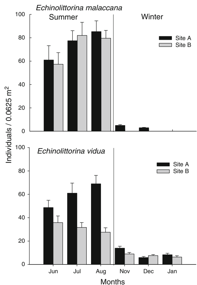
Fig. 2 Mean abundance (+SE) of Echinolittorina malaccana and E. vidua individuals in the barnacle habitats ( 25 \times 25 cm quadrats, n = 15 ) at two sites in Shek O during 3 months in summer and 3 months in winter
