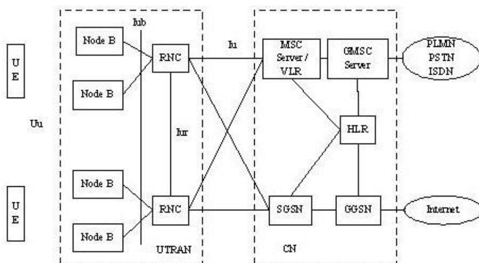
Figure 6: Network structure of TD-SCDMA [10]
