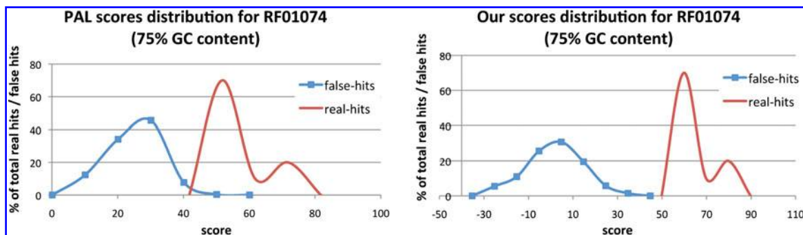
FIG. 5. Comparison the distribution between PAL scores and our scores for the families RF01074 for 75% GC-content random sequence.
