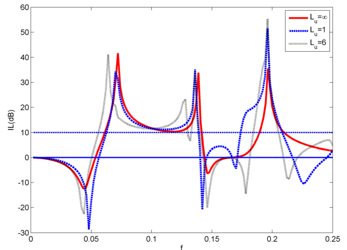
FIG. 9. (Color online) Variation of the IL against dimensionless frequency ( f ) for different duct lengths (dimensionless tension T = 0.05 , mass ratio m = 0.4 ).
