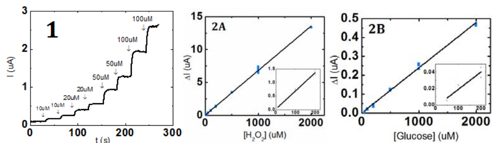
Figure 1: The amperometric i-t curve of addition of different [\text{H}_2\text{O}_2] .
