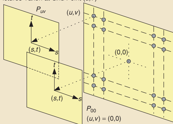
[FIG1] Concentric mosaic and lightfield.
