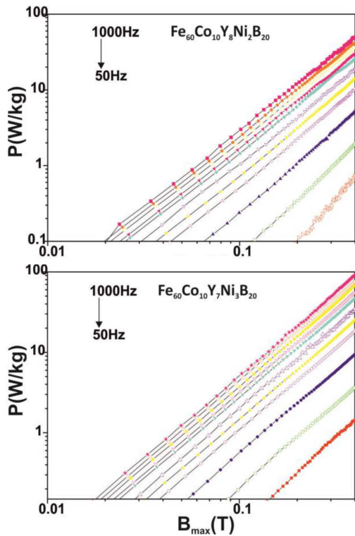
Fig. 6. Core losses as a function of the maximum induction for the produced alloys; tested over a magnetic field frequency range of 50–1000 Hz.
