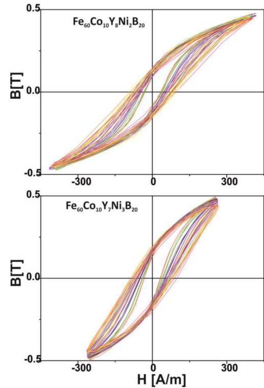
Fig. 4. Dynamic hysteresis loops, measured for the investigated alloys over a magnetic field frequency range of 50\text{--}1000 Hz.
