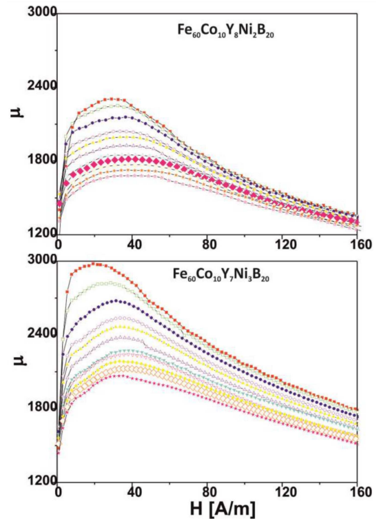
Fig. 5. Dependence of the magnetic permeability on the amplitude of the magnetising field; tested over a frequency range of 50\text{--}1000 Hz.
