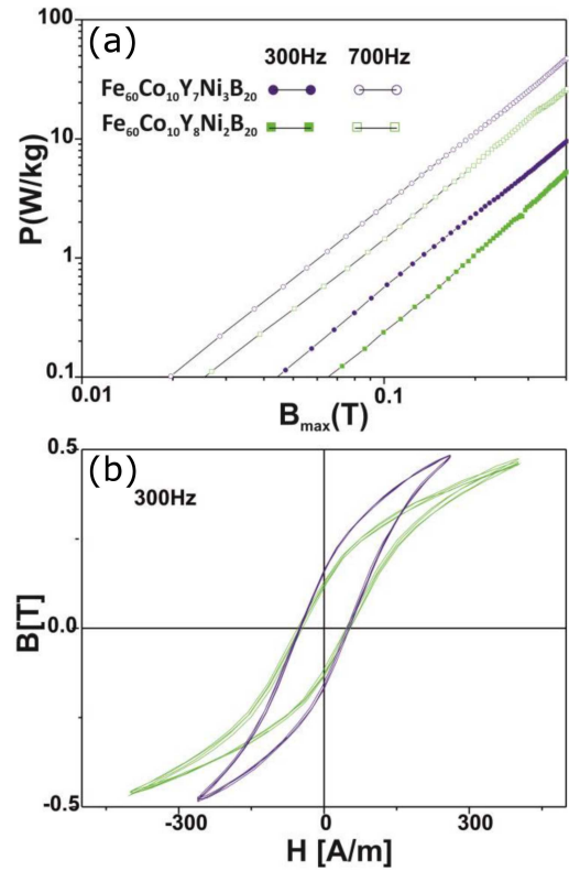
Fig. 7. Comparison of core losses (a) and dynamic magnetic hysteresis loops (b) for the produced alloys.
