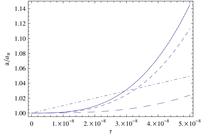
FIG. 9 (color online). Time variation of the scale factor of the finite temperature condensed dark matter for K_1 = 5 \times 10^{37} (solid curve), K_1 = 4 \times 10^{37} (dotted curve), K_1 = 2 \times 10^{37} (short dashed curve), K_1 = 0.6 \times 10^{37} (long dashed curve), and of the pressureless \Lambda CDM model (dash-dotted curve). The numerical values of the initial conditions and of the physical parameters are \theta_0 = 10^{-9} , a_{\text{tr}} = 10^{-4} , \chi_0 = 0.9999 , \kappa = 10^{15} , and \kappa_0 = 10^{10} .
