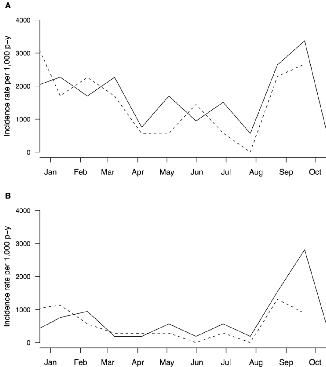
Appendix Figure 1. Incidence rates of acute upper respiratory tract infections in subjects who received trivalent inactivated influenza vaccine (TIV) or placebo. Panel (A) compares incidence rates of acute respiratory illness defined as at least two of body temperature \geq 37.8^{\circ}\text{C} , cough, sore throat, headache, runny nose, phlegm and myalgia; panel (B) compares incidence rates of febrile acute respiratory illness defined as body temperature \geq 37.8^{\circ}\text{C} plus cough or sore throat.
