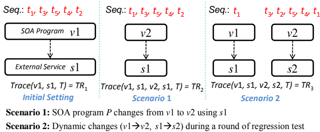
Figure 3. Two scenarios of test case execution sequences.
