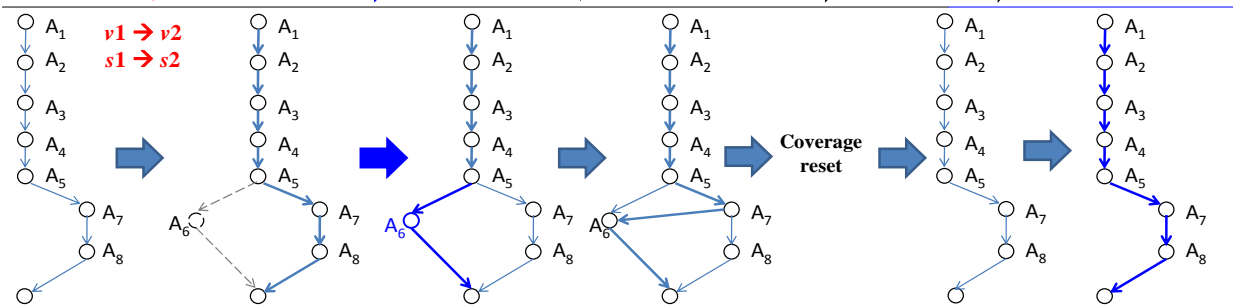
Figure 2. Brief example illustrating the preemptive regression testing of service-based applications.
