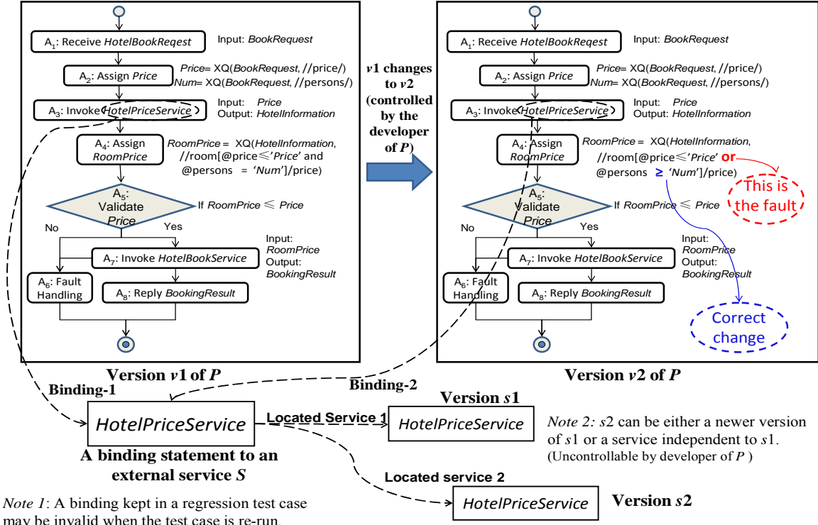
Figure 1. Brief example illustrating dynamic regression testing for dynamic SOA programs.
