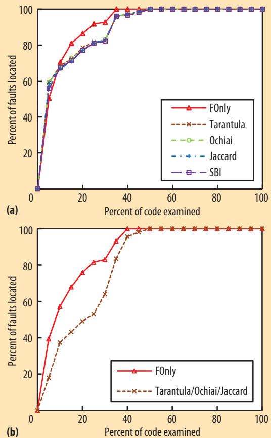
Figure 3. Fault-localization technique effectiveness: (a) pass-and-fail scenario and (b) fail-only scenario. When passed executions are unavailable or not reliable, FOnly's performance does not degrade as dramatically as peer techniques.
