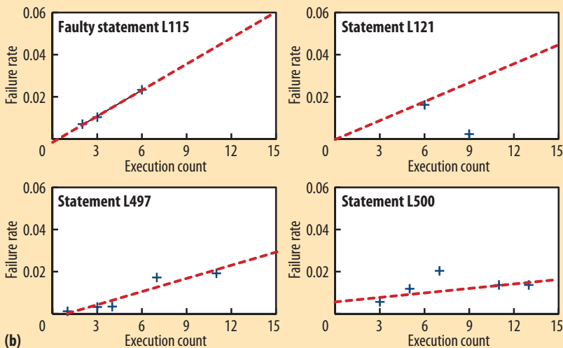
Figure 1. Applying the fault hypothesis to perform trend estimation. (a) Two code fragments from a faulty program. L121 is closer than L497 and L500 to the faulty statement, L115, in terms of the number of lines of code. (b) Plots of the failure rate versus the execution count for the four statements. As the execution count increases, the failure rates for L115 and L121 increase faster than those for L497 and L500.
