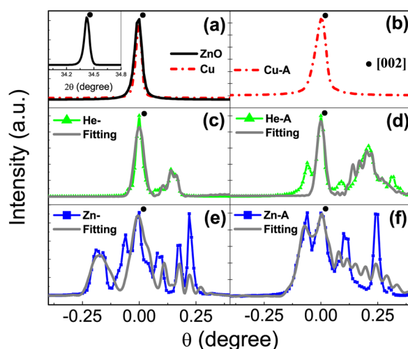
FIG. 4. (Color online) XRD rocking curves of the ZnO samples: (a) and (b) for Cu-implanted ZnO before and after thermal annealing, respectively; (c) and (d) for He-implanted; (e) and (f) for Zn-implanted. The solid line in Fig. 4(a) is for the as-grown ZnO. The inset in Fig. 4(a) shows XRD 2\theta scanning pattern of the as-grown ZnO. The solid lines (gray color) in (c), (d), (e), and (f) are the simulation results for the corresponding XRD rocking curves, respectively.
