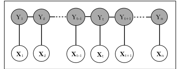
Figure 3: A graphical representation of a linear-chain CRF. For time step t , Y_t is a discrete hidden state, and X_t is an observation data vector. The feature function set is defined over the observation vector.
