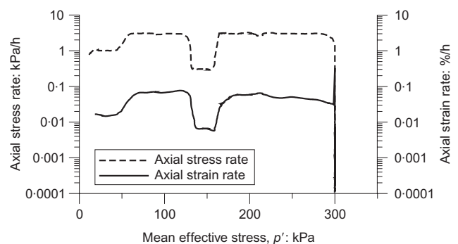
Fig. 3. Local axial strain rates measured during the isotropic compression LC-iso1 performed at constant rates of stress (3 and 0.3 kPa/h) on normally consolidated reconstituted London Clay.
