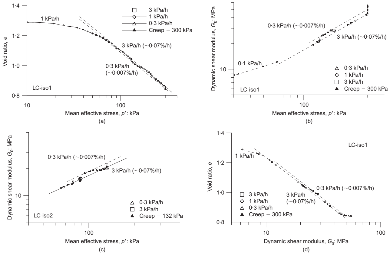
Fig. 9. Effect of changing the testing axial strain rate during isotropic compression of normally consolidated reconstituted London Clay: (a) e-\log p' (test LC-iso1); (b) and (c) \log G_0-\log p' (tests LC-iso1 and LC-iso2); (d) e-\log G_0 (test LC-iso1)
