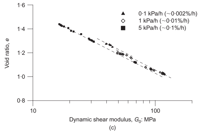
Fig. 8. Effect of changing the testing axial strain rate during isotropic compression of normally consolidated kaolin (test K-iso): (a) and (b) \log G_0 - \log p' ; (c) e - \log G_0
