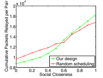
Fig. 5. Cumulative number of packets relayed per source-relay pair over levels of social closeness between the source-relay pair.
