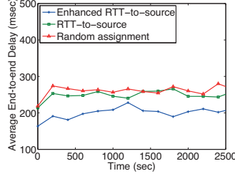
Fig. 7. End-to-end stream distribution delays: a comparison among three receiver-to-relay assignment methods.
