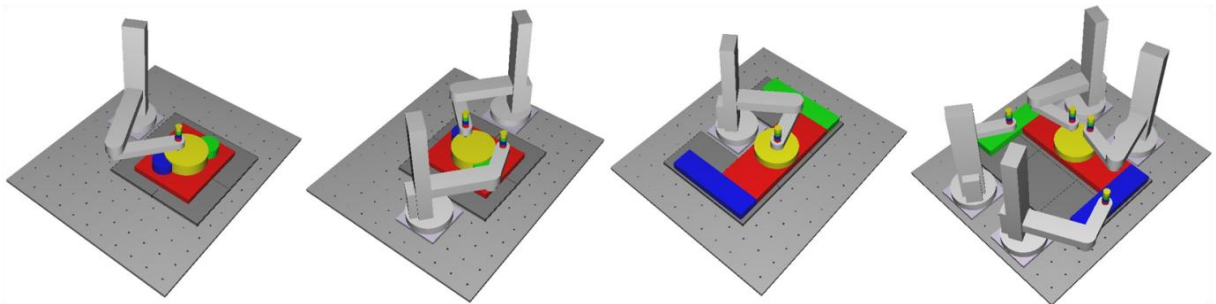
(a) Adjusting link lengths; (b) Dual modules operation; (c) C-style layout; (d) Multiple modules operation.
