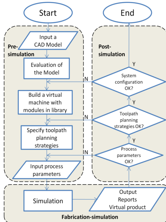
Fig. 2. Operation processes with the DRAMS
