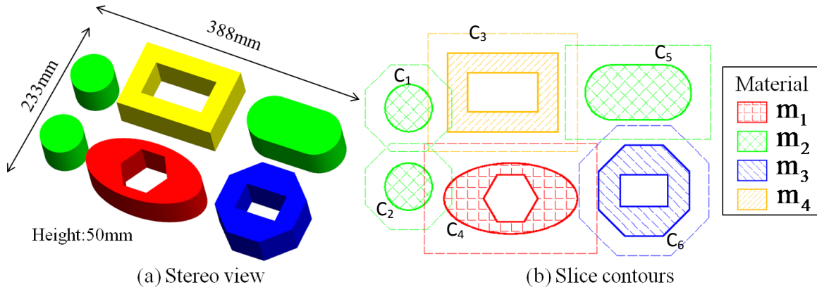
Fig. 7. A discrete multi-material sample part
