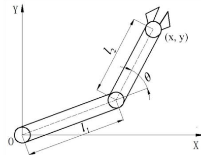
Fig. 6. A typical 2-DOF planar structure
