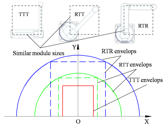
Fig. 5. Comparison of the work envelopes
