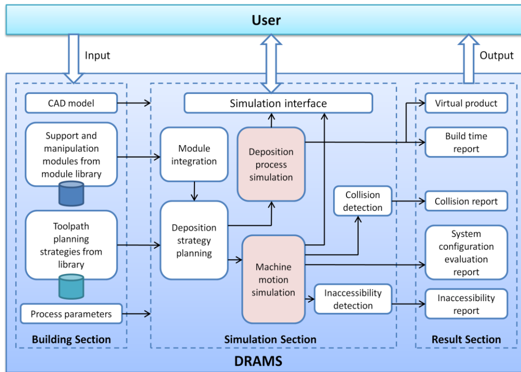
Fig. 1. Main elements and flow of the DRAMS
