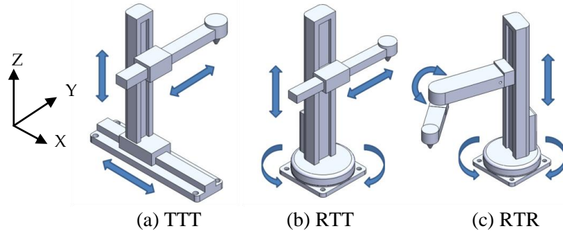
Fig. 4. Manipulation modules with common 3-DOF topologies
