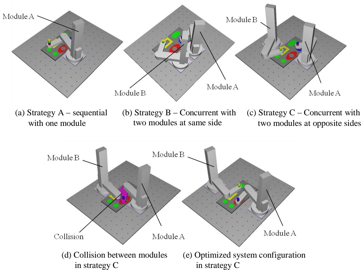
Fig. 8. Deposition strategies for the fabrication of the sample part
