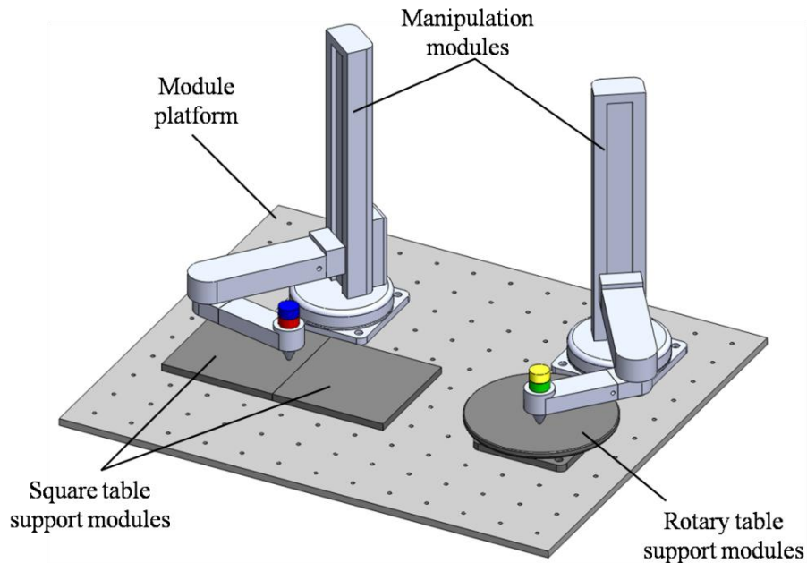
Fig. 3. A typical virtual reconfigurable AM machine in the DRAMS
