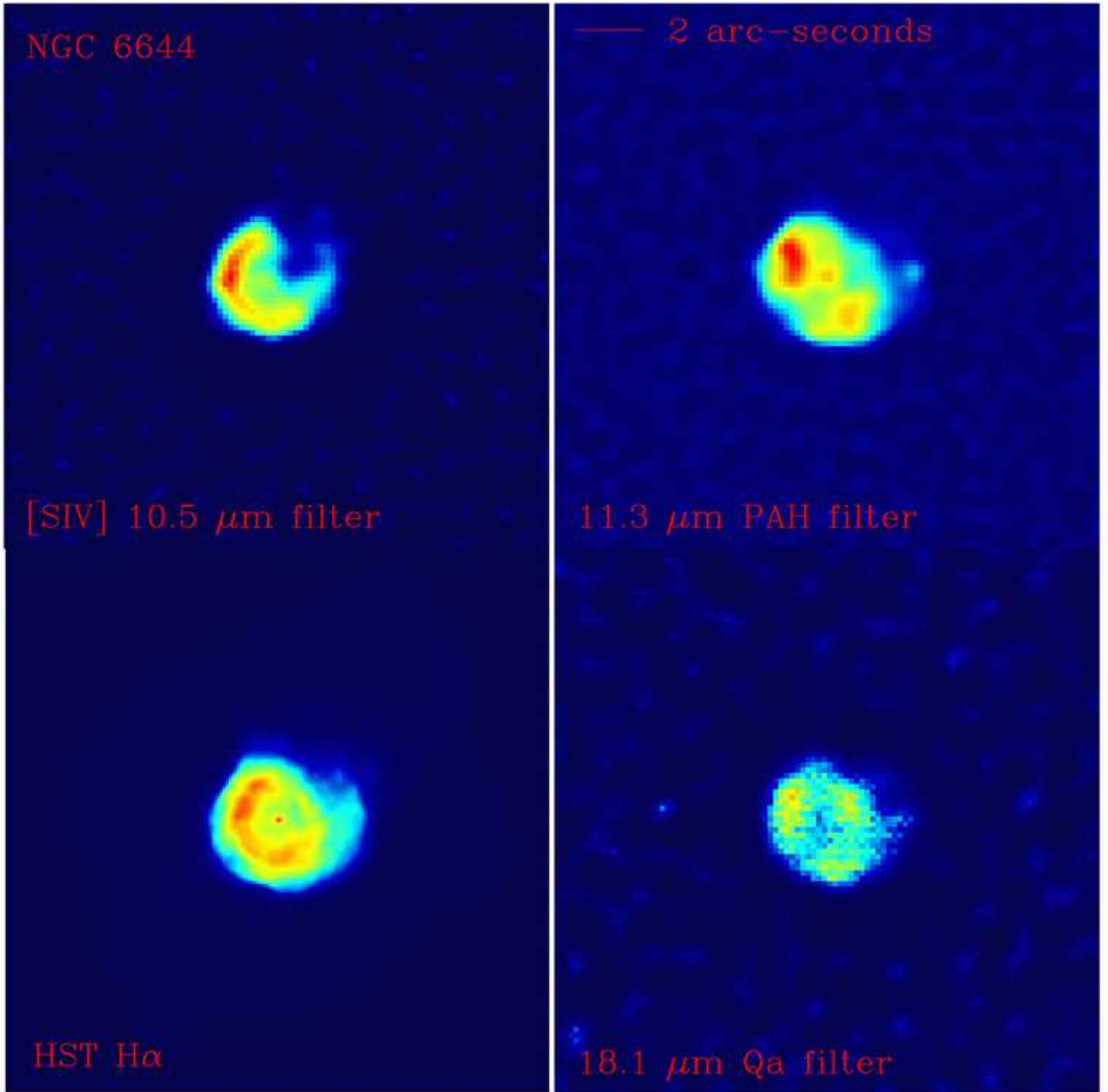
Fig. 9.— Comparison between the HST H\alpha image (lower left) and the flux-calibrated, deconvolved, false-color Gemini T-ReCS images displayed on the same pixel scale. The Gemini [S IV] 10.52\ \mu\text{m} narrow-band, PAH-2 11.3\ \mu\text{m} narrow-band, and the Q_a 18.3\ \mu\text{m} medium-band images are given in the upper left, upper right, and lower right panels respectively.
