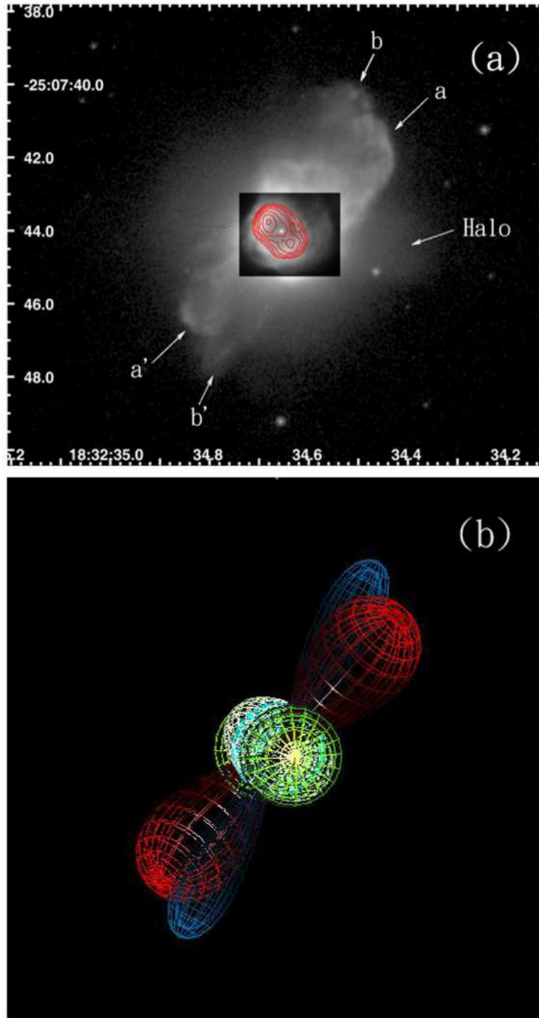
Fig. 12.— Comparison of optical-infrared observations and the three-dimensional model of NGC 6644. (a) The gray frame shows the HST H \alpha image, as in Figure 1. Linear contour plot of the T-ReCS PAH-2 11.3 \mu\text{m} image was overlaid on the HST image (red lines). (b) SHAPE three-dimensional mesh model. The bipolar lobes a , lobe b , and lobe c are displayed in red, blue, and green, respectively. The equatorial ring observed in the HST H \alpha image is shown in light blue and the infrared torus observed in Gemini PAH2 image is in white.
