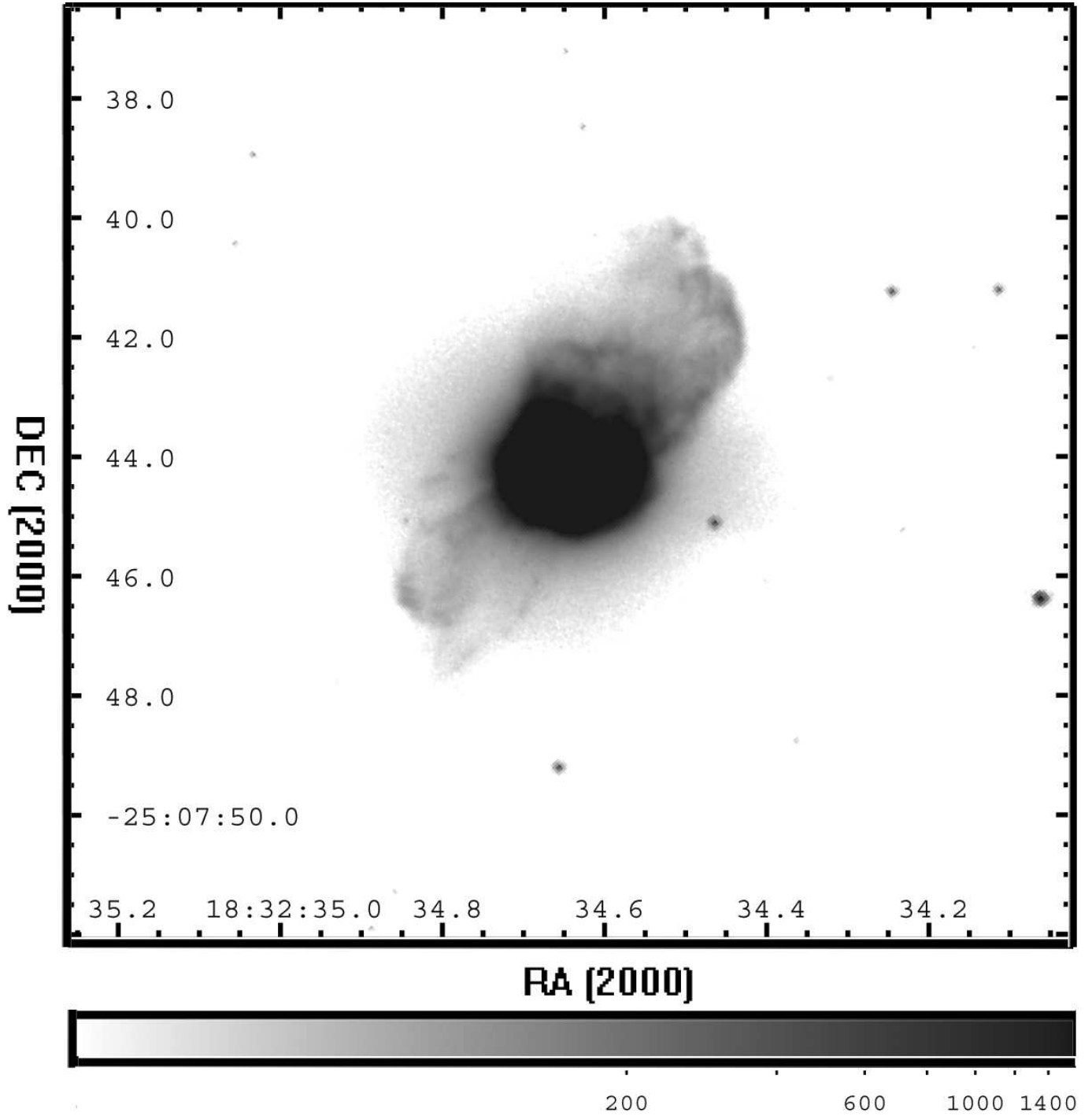
Fig. 4.— The HST H \alpha image of NGC 6644 with an intensity display setting to show the outer structures of the nebula. The intensity display is on a logarithmic scale and the grey scale bar is given at the bottom in units of counts per pixel.
