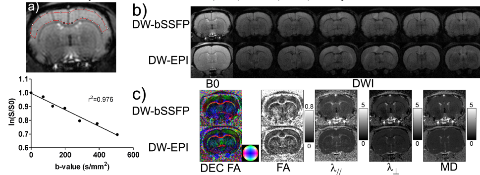
Fig. 3. a) By drawing an ROI on the cortex and plotting the signal intensity against b-value, the signal decay is nearly monoexponential to the b-value. b) DWIs along 6 different directions and B0 images using DW-bSSFP and DW-EPI. Note that the diffusion attenuation of anisotropic white matter varies with the direction of applied diffusion gradient. c) DTI parametric maps (directionally encoded colour FA, \lambda_{//} , \lambda_{\perp} , MD). Unit of diffusivities are mm 2 /ms.
