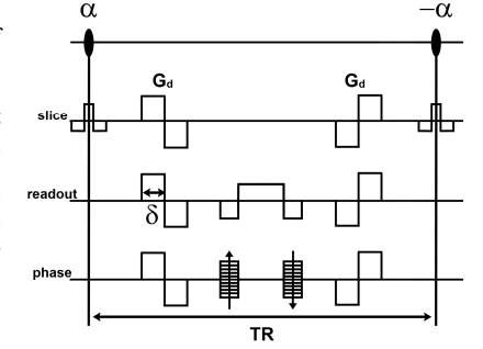
Fig. 1. Proposed DW bSSFP sequence with two bipolar gradients ( G_d ) inserted with TE=TR/2 . All the imaging and diffusion gradients are balanced.
