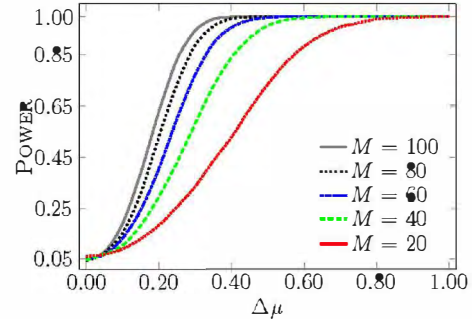
Figure 6: The relationship among the power of \hat{\theta} , the location shift parameter \Delta\mu and the sample size M .
