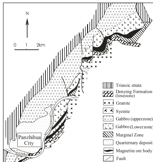
Figure 1. Geological map of the Panzhihua layered intrusion, SW China.
