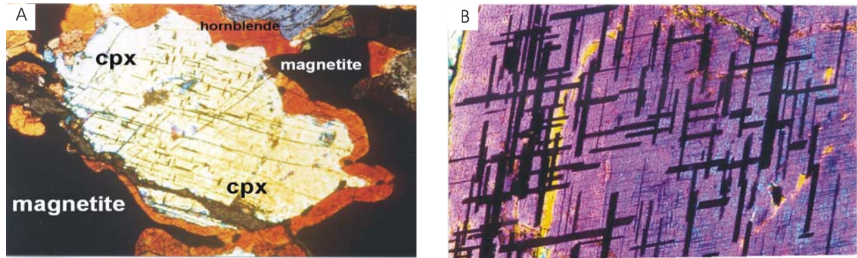
Figure 2. Microphotos of gabbros from the Panzihua intrusion: A) Hornblende rimming clinopyroxene. B) Clinopyroxene with ilmenite exsolution lamellae.
