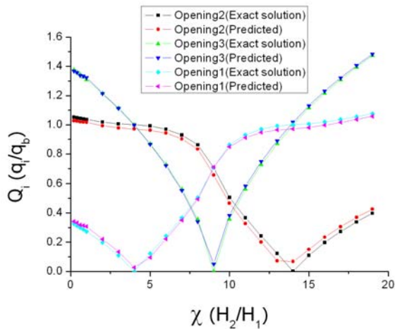
Figure6. Comparison of predicted normalized airflow rates through three openings using MIX and the theoretical solution ( Fr=2 , wind is approaching from right to left)
