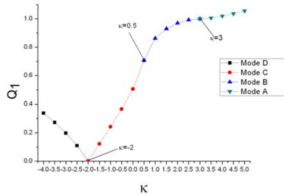
Figure4 All possible airflow modes for Opening 1
