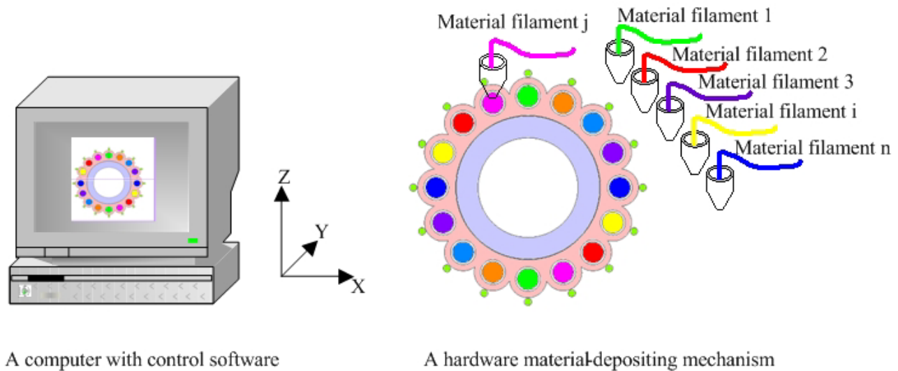
Fig. 1. A layer of a multi-material part being fabricated
