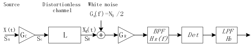
Fig.1 Signal transmission link
