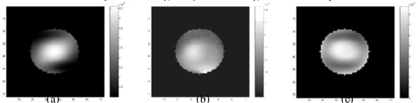
Fig.2 Simulated images of sphere phantom on the central axial plane (a) Shielded Birdcage coil, (b) TEM coil, (c) Microstrip coil. The average relative SNR for shield Birdcage, TEM and Microstrip coils are 1, 1.14, and 1.58 respectively.
