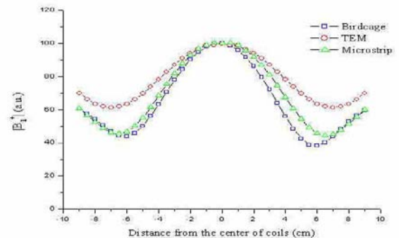
Fig.1 Simulated |B_1^+| field distributions in the transverse direction for loaded volume coils. Amplitudes of B_1^+ field at the center of all coils are normalized to 100%. TEM has better loaded B_1^+ field homogeneity than Birdcage and Microstrip coils
