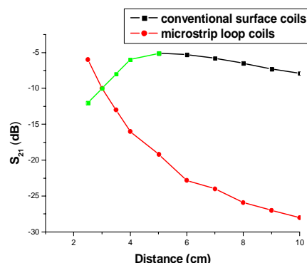
Fig. 2 S_{21} measurement of two coils side by side: (1) conventional surface coils; (2) microstrip loop coils
