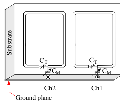
Fig. 1 Structure of a 2-element MLA
