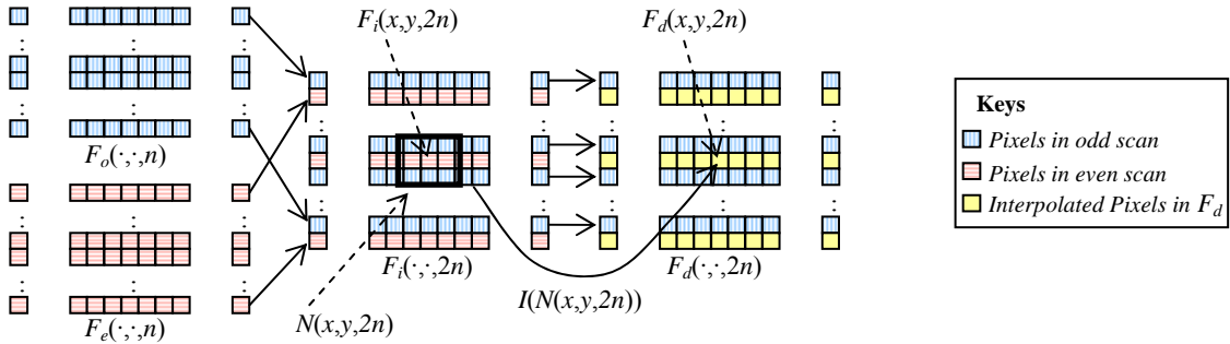
Fig. 2. Relationship between F_o(\cdot, n) , F_e(\cdot, n) and F_i(\cdot, 2n) . F_d(x, y, 2n) is reconstructed by interpolating the pixels within N(x, y, 2n) .
