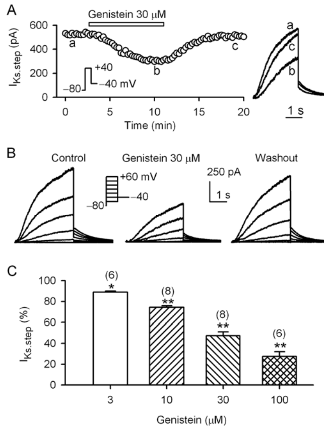
Fig. 1. Effect of genistein on the recombinant I_{K_s} . A. Time-course of the recombinant I_{K_s} recorded in a typical experiment with 3-s voltage step to +40 from -80 mV, then back to -40 mV (to recorded I_{K_s} tail current) as shown in the inset in the absence and presence of 30 \mu\text{M} genistein. Original I_{K_s} traces at corresponding time points are shown in right of the panel. B. Voltage-dependent I_{K_s} traces recorded in a representative cell with 3-s voltage steps to between -60 and +60 mV from -80 mV (20-mV increment, 0.05 Hz), then to -40 mV ( inset ) in the absence and presence of 30 \mu\text{M} genistein. Genistein reversibly inhibited the voltage-dependent current. C. Mean percent value of the recombinant I_{K_s} (at +40 mV) inhibition by 3, 10, 30 and 100 \mu\text{M} genistein. The number in the parenthesis indicates the experimental number. * P < 0.05 ; ** P < 0.01 vs control.
