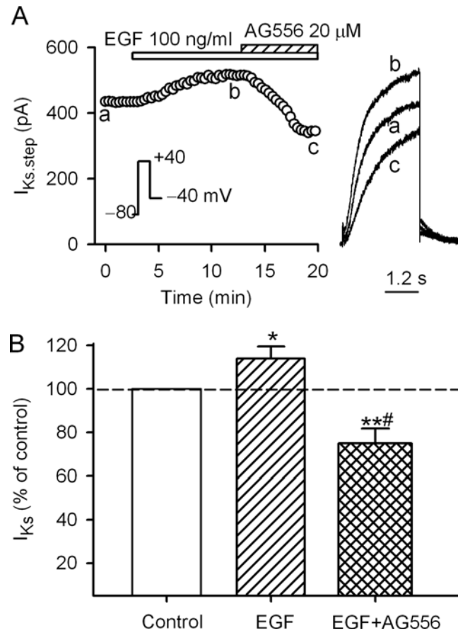
Fig. 6. EGF enhanced the recombinant I_{Ks} in cells with serum-free culture. A. Time-course of I_{Ks} recorded in typical experiment in the absence and presence of 100 ng/ml EGF and after co-application of EGF and 20 \mu M AG556. Original current traces at corresponding time points are shown in right of the panel. B. Histogram showing the mean percent values of the recombinant I_{Ks} (at +40 mV) in cells with a 36-h serum-free culture during control, in the presence of 100 ng/ml EGF and after co-application of EGF and 20 \mu M AG556. n = 6 , * P < 0.05 , ** P < 0.01 vs control; # P < 0.01 vs EGF alone.
