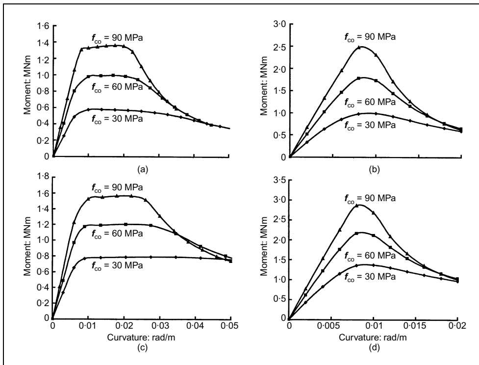
Fig. 4. Complete moment–curvature curves of some beam sections analysed: (a) under-reinforced and with no compression reinforcement ( \rho_t/\rho_b = 0.5 , \rho_c = 0\% ); (b) over-reinforced and with no compression reinforcement ( \rho_t/\rho_b = 1.5 , \rho_c = 0\% ); (c) under-reinforced and with compression reinforcement ( \rho_t/\rho_b = 0.5 , \rho_c = 1\% ); (d) over-reinforced and with compression reinforcement ( \rho_t/\rho_b = 1.5 , \rho_c = 1\% )
