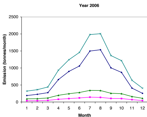
Figure 2. Monthly BVOC emissions in 2006.
