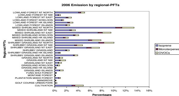
Figure 5. 2006 Emission breakdown by PFTs.
