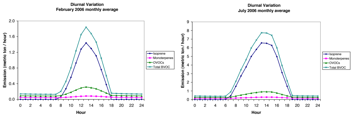
Figure 1. Diurnal variation of BVOC emission in February and July 2006
