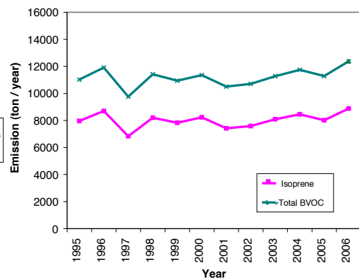
Figure 3. Annual BVOC emissions from 1995 to 2006.
