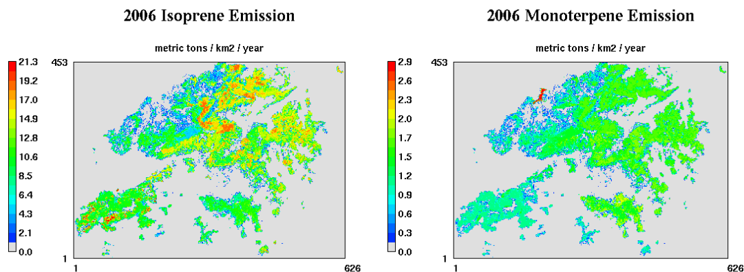
Figure 4. Spatial variation of BVOC emissions in 2006 (a) Isoprene; (b) Monoterpene.
