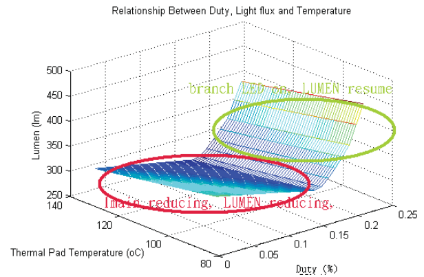
Fig 7 The overall Light flux versus Temperature and duty cycle
