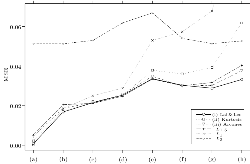
Figure 3. MSE's of L_p estimators under various error densities : (a) \zeta = 0.3 ; (b) \zeta = 0.8 ; (c) upwardly pointed, \zeta = 1, q = 0.25 ; (d) upwardly pointed, \zeta = 1, q = 2 ; (e) downwardly pointed, \zeta = 1, q = 0.25 ; (f) downwardly pointed, \zeta = 1, q = 2 ; (g) \zeta = 1.3 ; and (h) \zeta = 1.8 .
