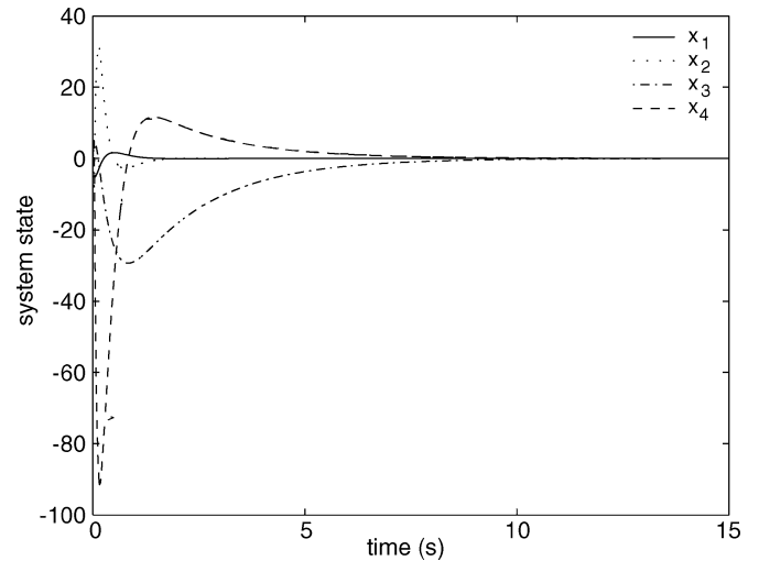
Fig. 5. Initial condition response of the closed-loop system.
