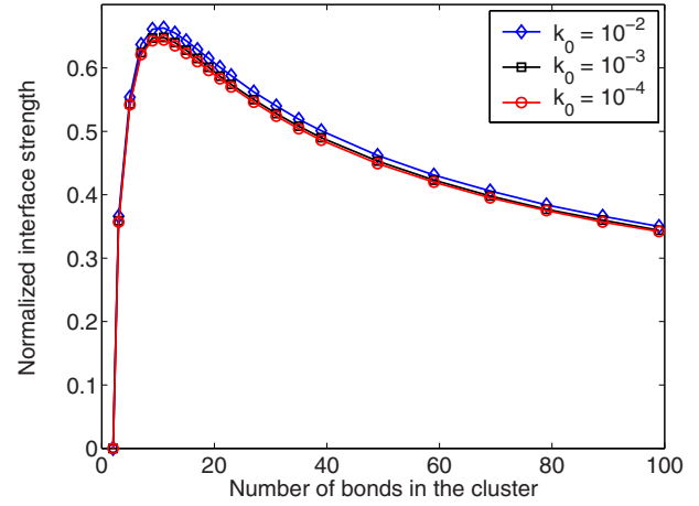
FIG. 4. (Color online) Normalized interface strength 2b\sigma_\infty^{max}/f_0C_b as a function of cluster size.
