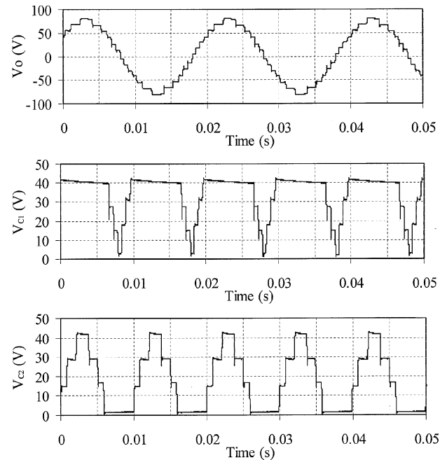
Fig. 6. Measured waveforms.
