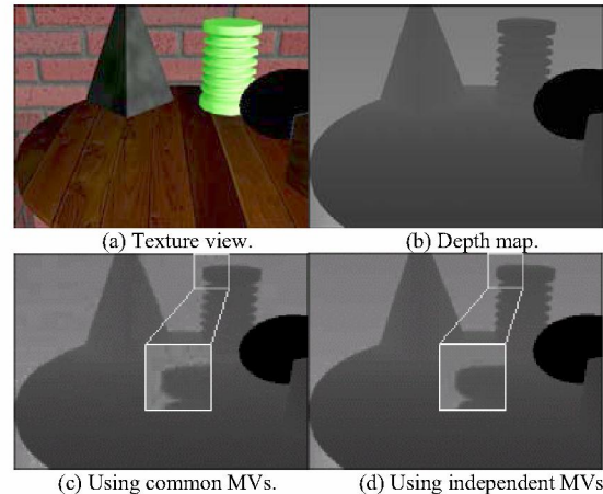
(c) Using common MVs. (d) Using independent MVs Fig. 6. An example of depth coding results for a VOP in a dynamic lighting environment
