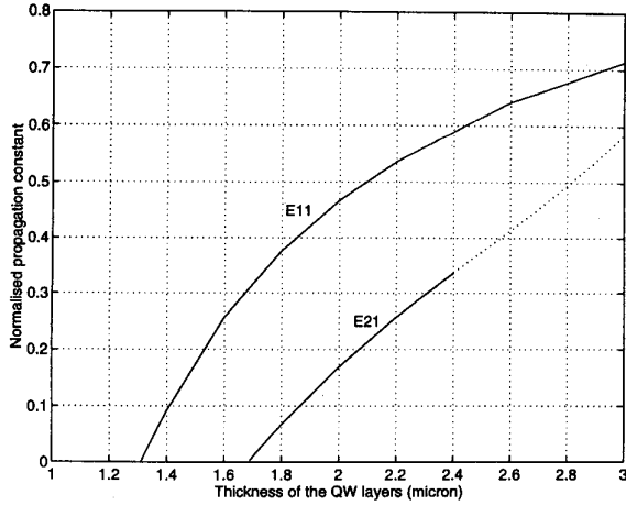
Fig. 4. Normalised propagation constant as a function of thickness of the QW layers with mask width of 1.5\mu\text{m} and operating wavelength at 0.9\mu\text{m} .
