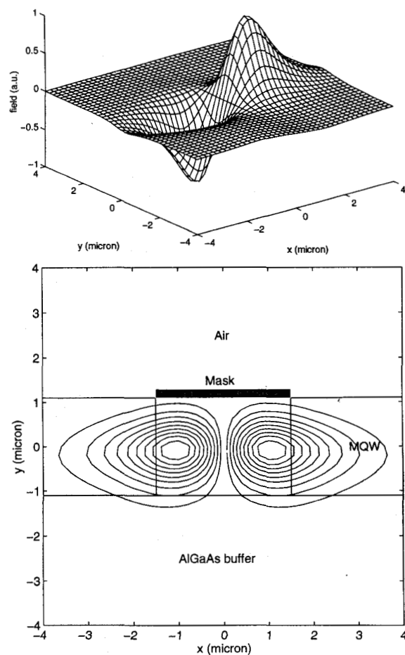
Fig. 6. Antisymmetric E_{21} field profile as determined by FDM with QW layers thickness of 2.2\mu m . Contour levels are at 10% intervals of the maximum field amplitude.
