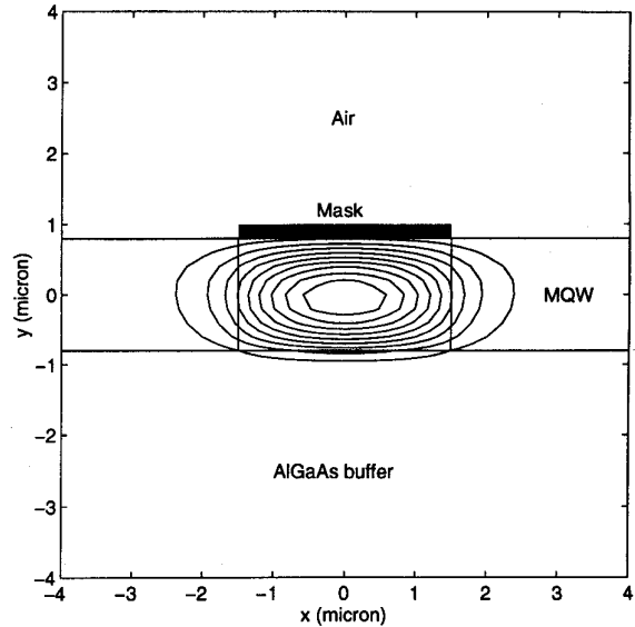
Fig. 5. Symmetric E_{11} field profile as determined by FDM with QW layers thickness of 1.6\mu\text{m} . Contour levels are at 10% intervals of the maximum field amplitude.
