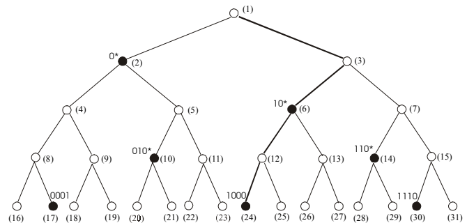
Figure 1. A binary-trie for a 4-bit address space.
