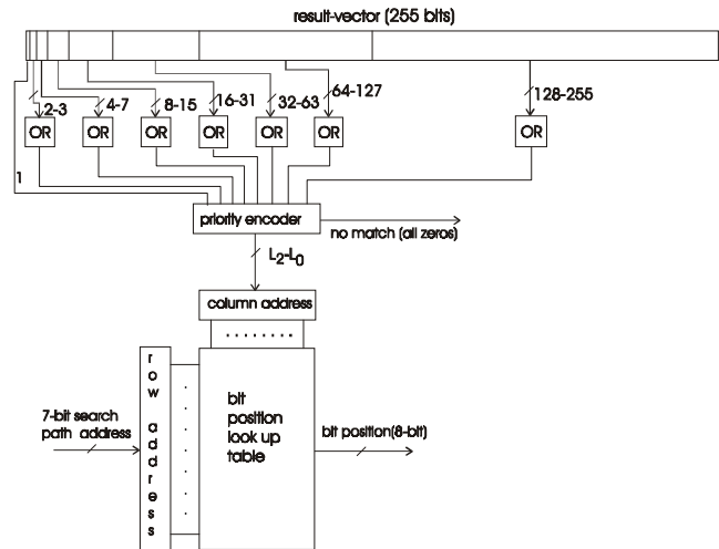
Figure 3. Organization of the RMB locator .
