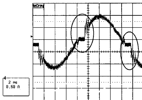
Fig. 1. Crossover distortion
