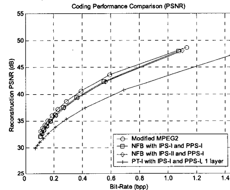
Fig. 6. Coding results of the light field Dragon .
