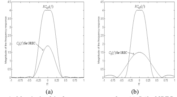
Figure 1. Magnitude of the frequency responses for (a) C_0(f) of 3REC and RC_{4T}(f) (b) C_0(f) of 1REC and RC_{4T}(f)
