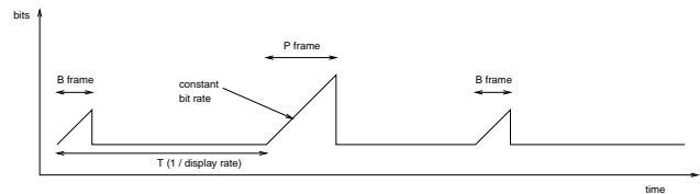
Fig. 4. Scheduling video frames using a periodic approach.
