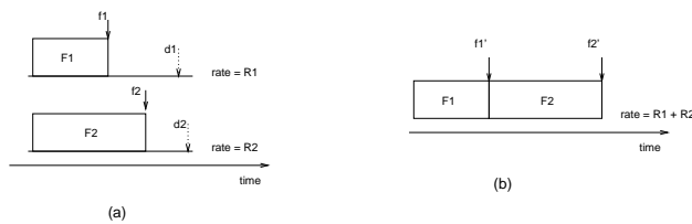
Fig. 5. (a) Rate based scheduling; (b) time-division based scheduling.
