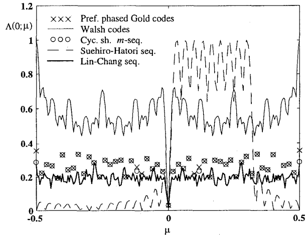
Fig. 2. Worst-case time-frequency crosscorrelation \Lambda(0;\mu) .
